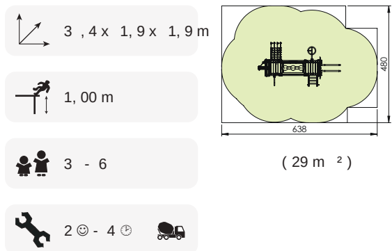
G510 (stainless steel tubes)
